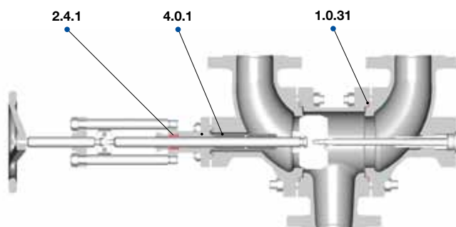
Spare parts, gasket set complete
