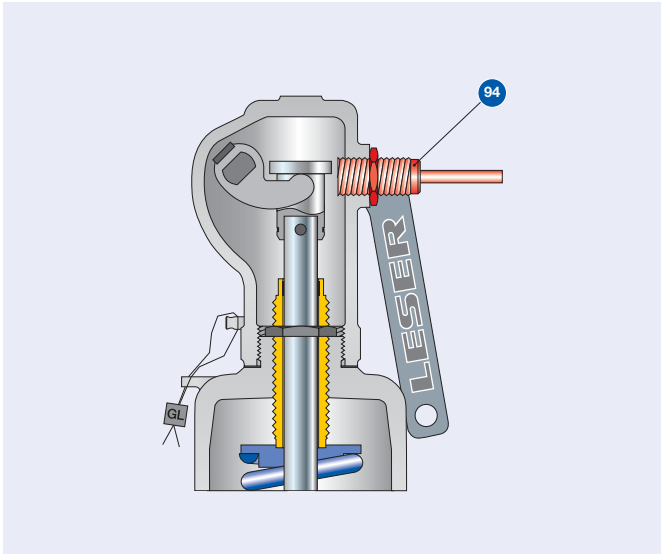
Packed lever H4
