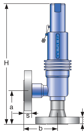
Balanced bellows
