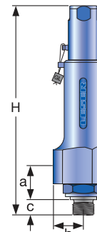
Long version – male thread
