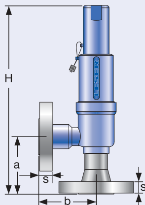
Conventional design
